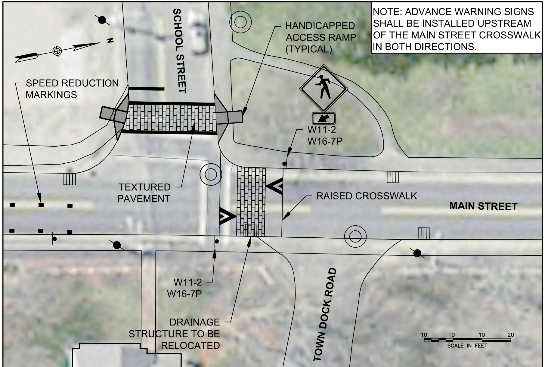
Concept Plan 4 - Main Street at School Street Long-Term Improvements Cotuit, MA
